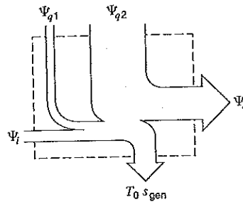
FIGURE 10.16 Fluxes, flows, and destruction of exergy in the feedwater heater.
