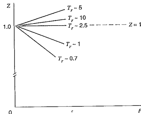
FIGURE 13.5 Low-pressure region of compressibility chart.
