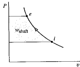
FIGURE 9.7 Shaft work from Eq. 9.18.
