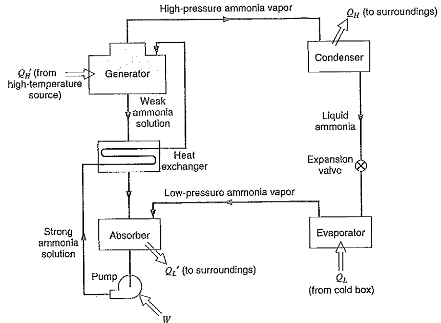
FIGURE 11.35 The ammonia-absorption refrigeration cycle.
