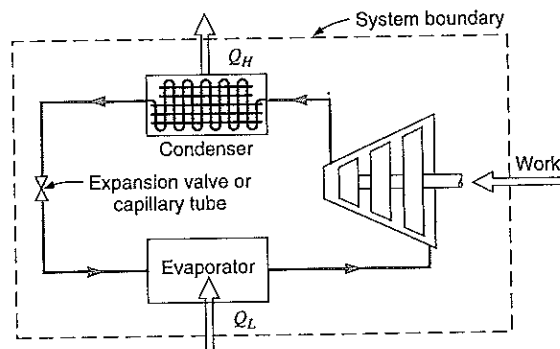
FIGURE 7.6 A simple refrigeration cycle.
