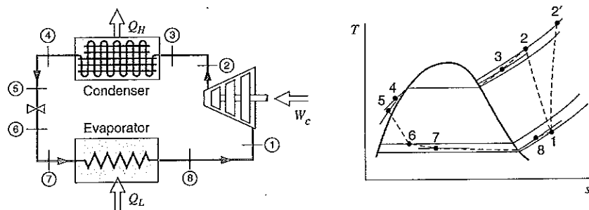
FIGURE 11.34 The actual vapor-compression refrigeration cycle.
