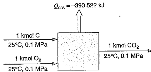
FIGURE 14.3 Example of combustion process.
