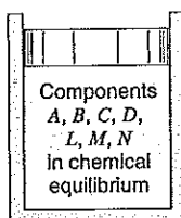
FIGURE 15.10 Sketch demonstrating simultaneous reactions.
