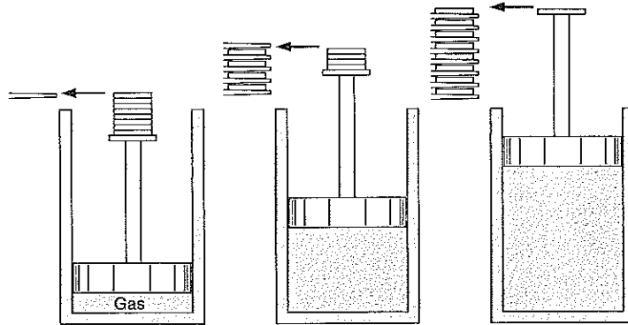
FIGURE 7.13 An example of a process that approaches being reversible.
