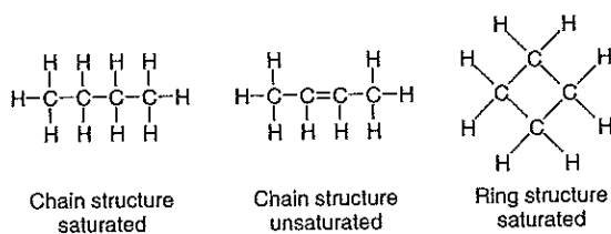
FIGURE 14.1 Molecular structure of some hydrocarbon fuels.
