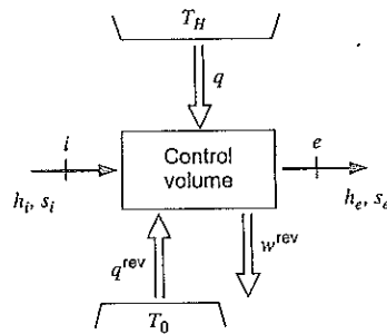
FIGURE 10.5 An ideal reversible process.
