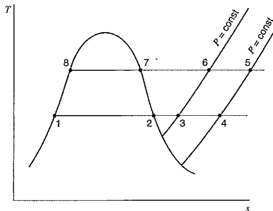
FIGURE 13.11 Sketch showing procedure for developing a table of thermodynamic properties from experimental data.
