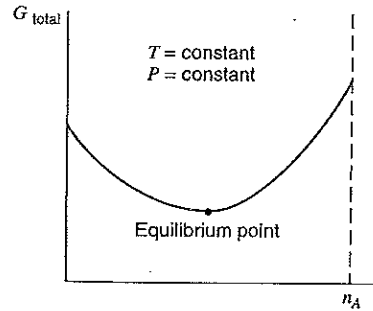
FIGURE 15.3 Illustration of the requirement for chemical equilibrium.
