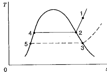
FIGURE 12.4 Temperature–entropy diagram to show the cooling of a gas–vapor mixture at a constant pressure.
