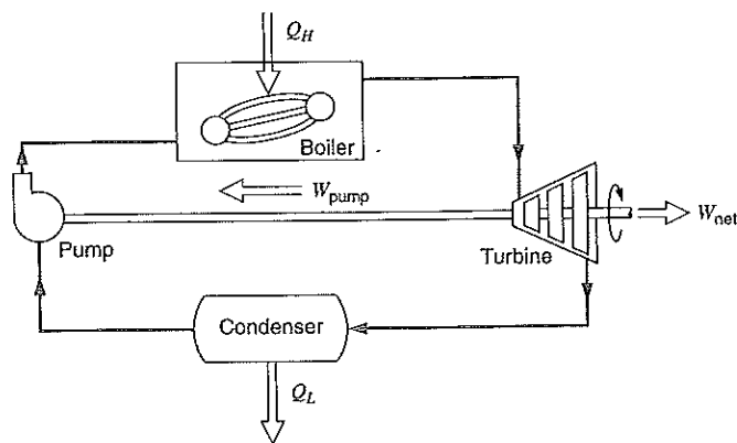
FIGURE 9.8 Simple steam power plant.
