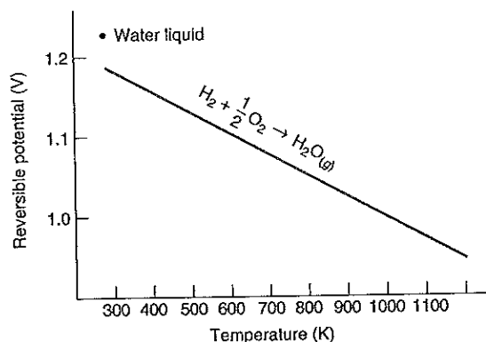
FIGURE 14.7 Hydrogen–oxygen fuel cell ideal EMF as a function of temperature.
