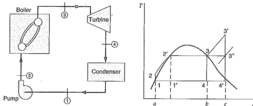
FIGURE 11.3 Simple steam power plant that operates on the Rankine cycle.
