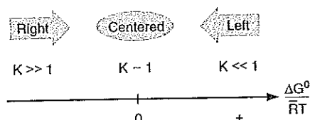
FIGURE 15.8 The shift in the reaction with the change in Gibbs function.
