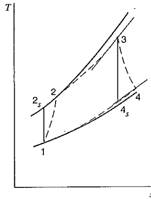
FIGURE 11.20 Effect of inefficiencies on the gas-turbine cycle.
