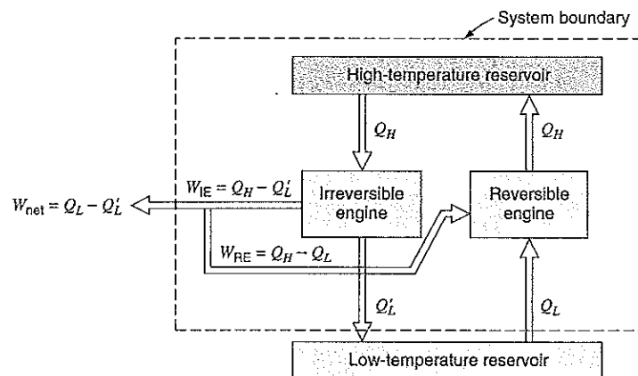
FIGURE 7.20 Demonstration of the fact that the Carnot cycle is the most efficient cycle operating between two fixed-temperature reservoirs.
