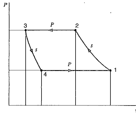
FIGURE 11.32 Four-process refrigeration cycle.
