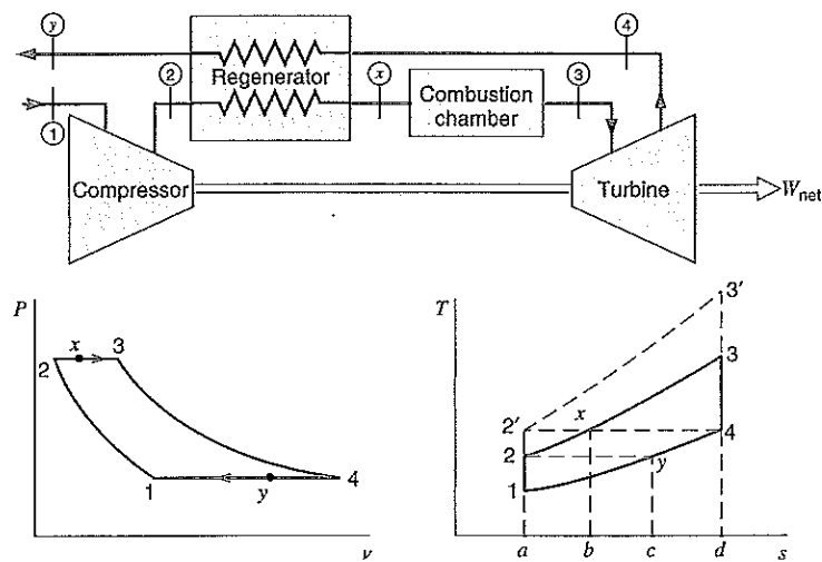
FIGURE 11.21 The ideal regenerative cycle.
