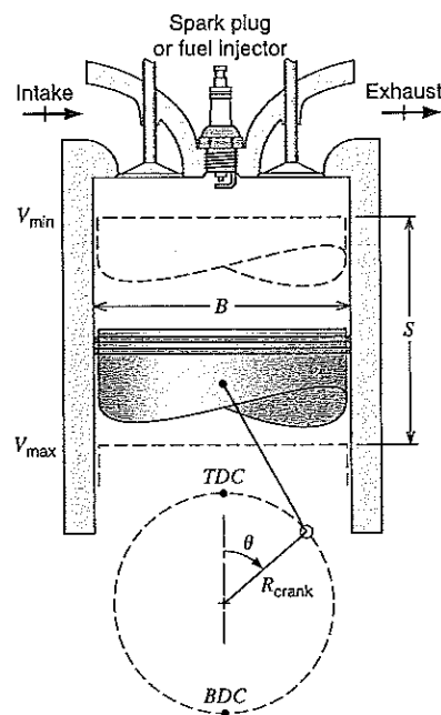
FIGURE 11.27 The piston-cylinder configuration for an internal combustion engine.
