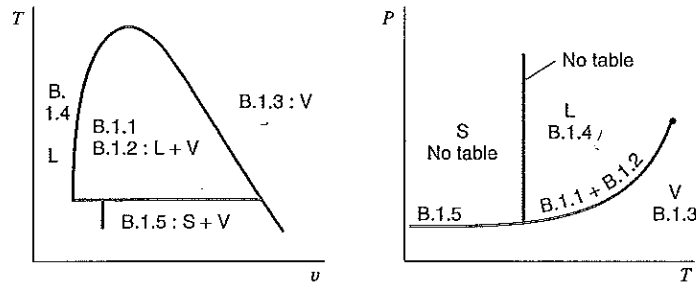
FIGURE 3.8 Listing of the steam tables.
