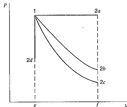
FIGURE 4.8 Pressure-volume diagram showing work done in the various processes of Example 4.1.
