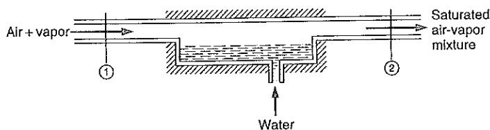
FIGURE 12.6 The adiabatic saturation process.
