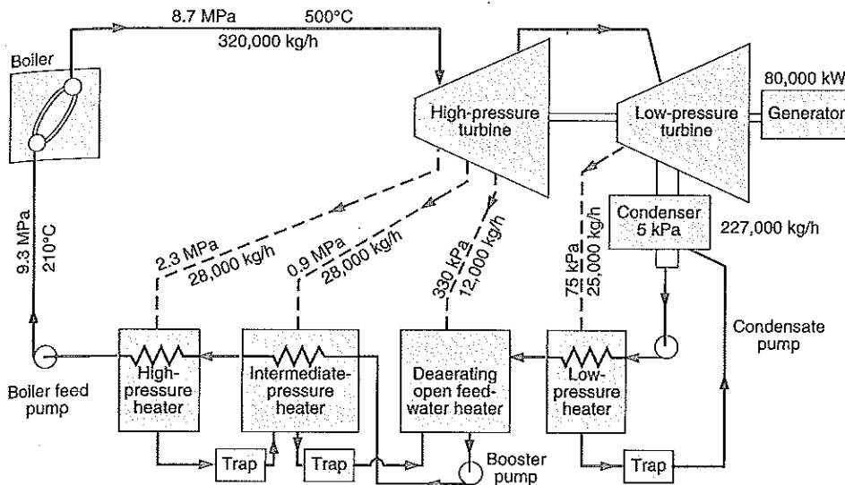
FIGURE 11.12 Arrangement of heaters in an actual power plant utilizing regenerative feedwater heaters.
