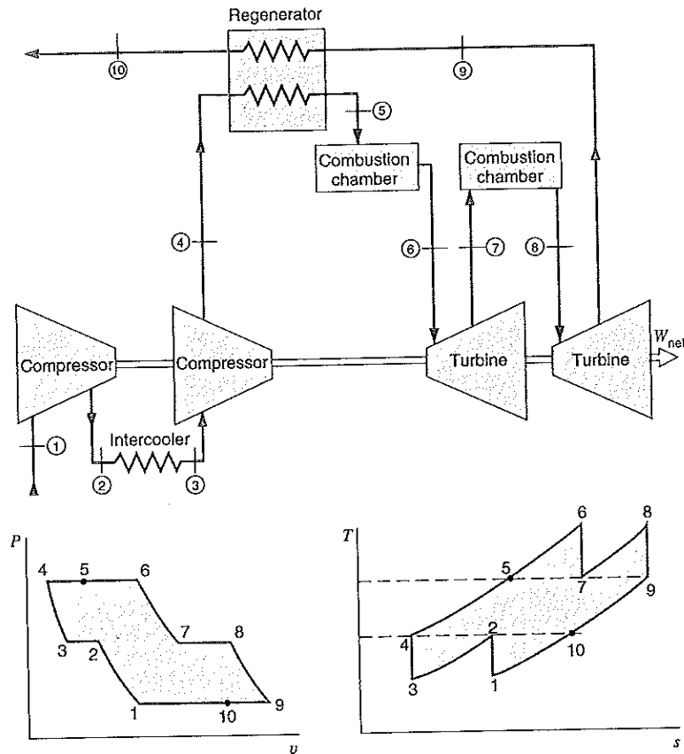
FIGURE 11.23 The ideal gas-turbine cycle utilizing intercooling, reheat, and a regenerator.
