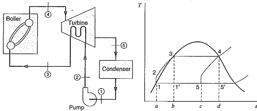
FIGURE 11.9 The ideal regenerative cycle.
