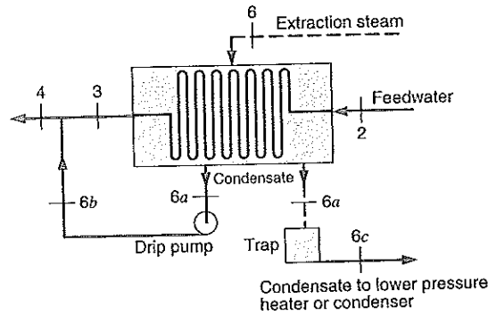
FIGURE 11.11 Schematic arrangement for a closed feedwater heater.
