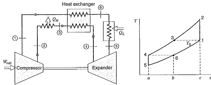
FIGURE 11.38 The air-refrigeration cycle utilizing a heat exchanger.
