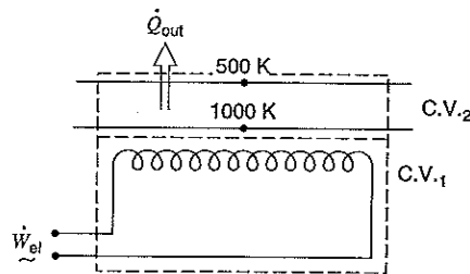
FIGURE 10.17 The electric heating element and ceramic top of a stove.
