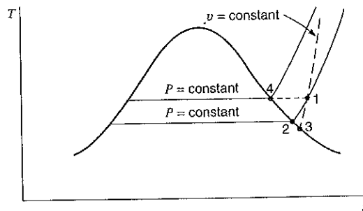
FIGURE 12.3 Temperature–entropy diagram to show definition of the dew point.
