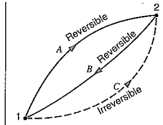
FIGURE 8.12 Entropy change of a control mass during an irreversible process.
