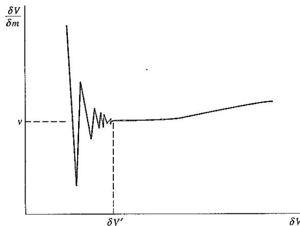
FIGURE 2.6 The continuum limit for the specific volume.
