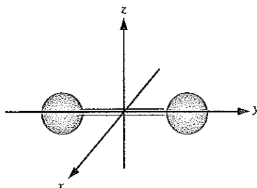
FIGURE 2.4 The coordinate system for a diatomic molecule.
