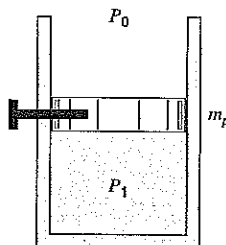
FIGURE 4.14 Example of a nonequilibrium process.
