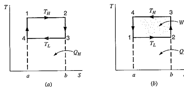
FIGURE 8.8 The Carnot cycle on the temperature–entropy diagram.
