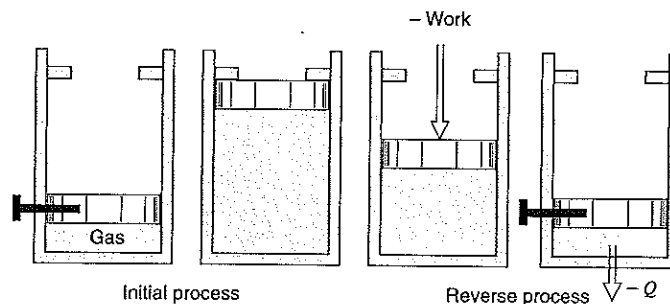
FIGURE 7.12 An example of an irreversible process.
