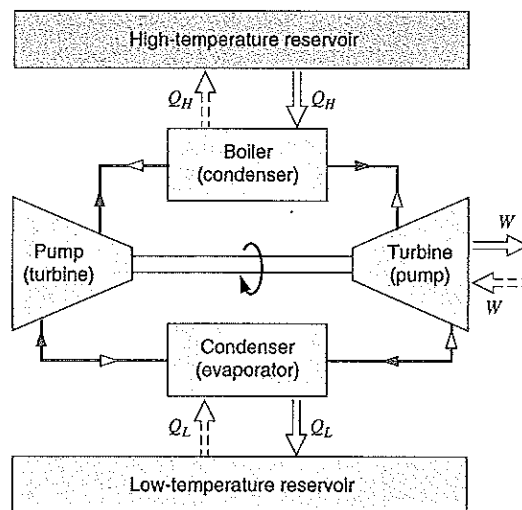
FIGURE 7.18 Example of a heat engine that operates on a Carnot cycle.
