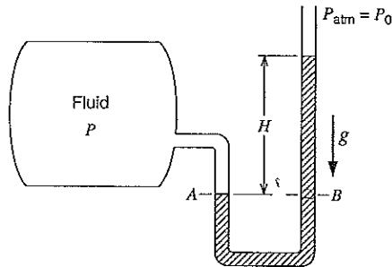
FIGURE 2.12 Example of pressure measurement using a column of fluid.
