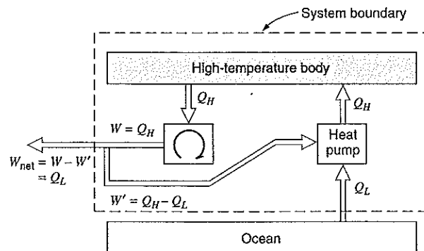
FIGURE 7.11 A perpetual-motion machine of the second kind.
