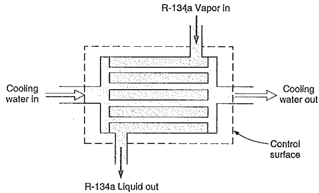
FIGURE 6.6 Schematic diagram of an R-134a condenser.
