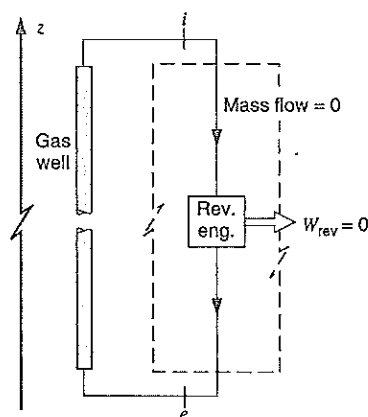
FIGURE 15.2 Illustration showing the relation between reversible work and the criteria for equilibrium.
