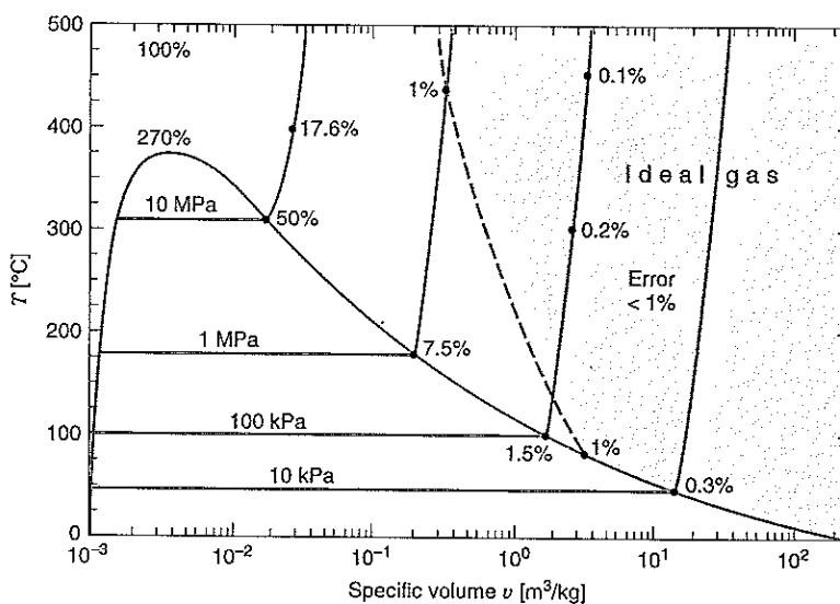
FIGURE 3.21 Temperature-specific volume diagram for water.
