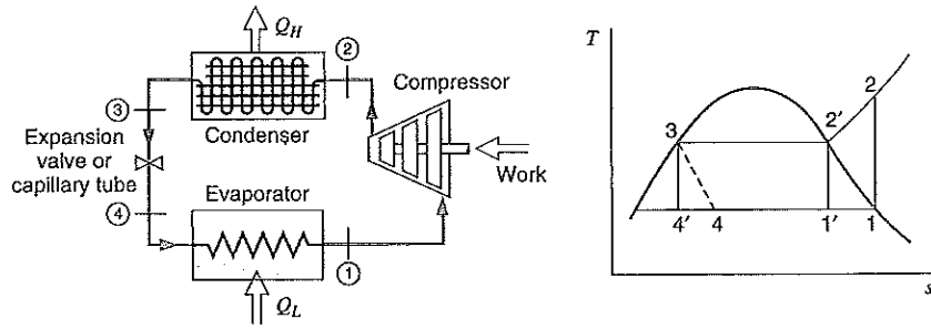
FIGURE 11.33 The ideal vapor-compression refrigeration cycle.
