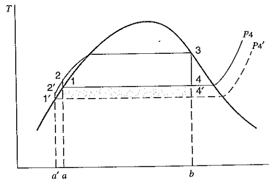
FIGURE 11.4 Effect of exhaust pressure on Rankine-cycle efficiency.
