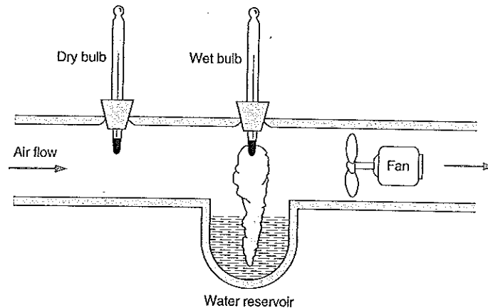
FIGURE 12.7 Steady-flow apparatus for measuring wet- and dry-bulb temperatures.
