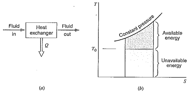
FIGURE 10.3 Changing-temperature energy source.
