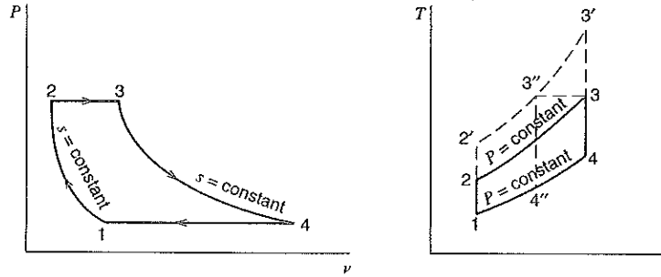
FIGURE 11.19 The air-standard Brayton cycle.
