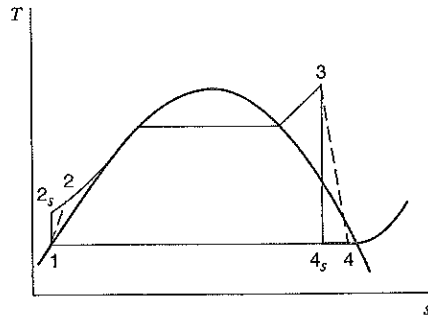
FIGURE 11.13 Temperature–entropy diagram showing effect of turbine and pump inefficiencies on cycle performance.
