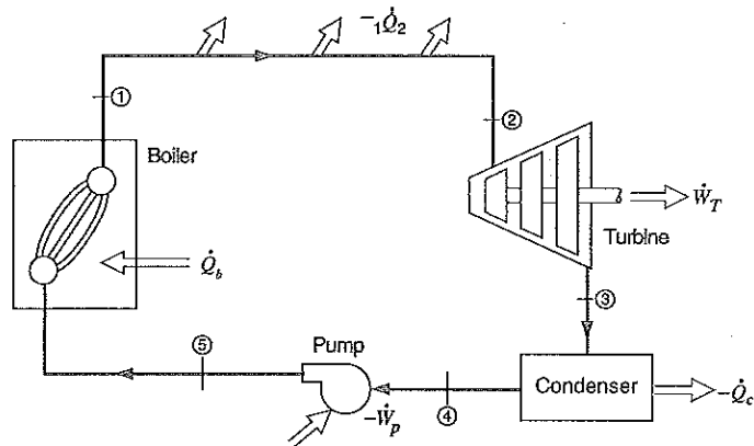
FIGURE 6.12 Simple steam power plant.
