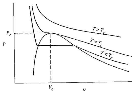
FIGURE 13.7 Plot of isotherms in the region of the critical point on pressure-volume coordinates for a typical pure substance.
