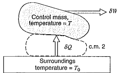
FIGURE 8.15 Entropy change for the control mass plus surroundings.
