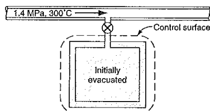
FIGURE 6.14 Flow into an evacuated vessel—control volume analysis.
