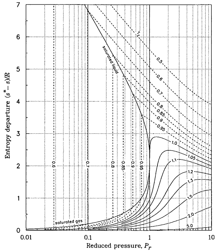
FIGURE D.3 Lee-Kesler Simple Fluid Entropy Departure.
