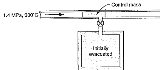
FIGURE 6.15 Flow into an evacuated vessel—control mass.
