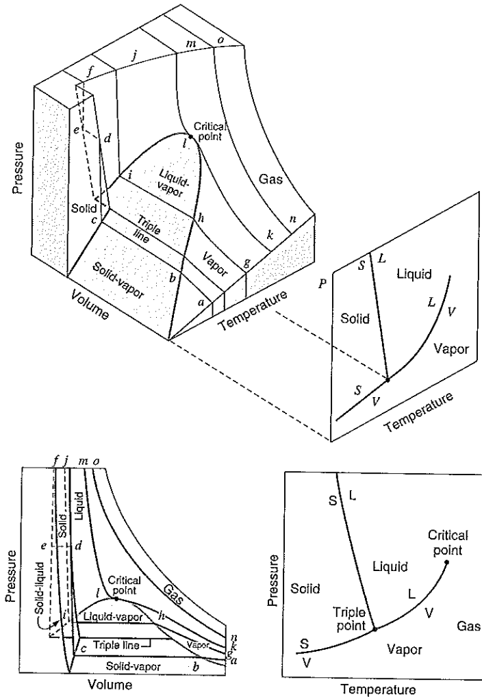
FIGURE 3.18 Pressure-volume-temperature surface for a substance that expands on freezing.
