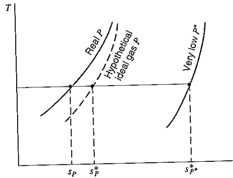
FIGURE 13.9 Real and ideal gas states and entropies.
