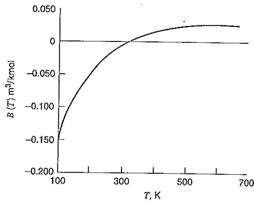
FIGURE 13.6 The second virial coefficient for nitrogen.
