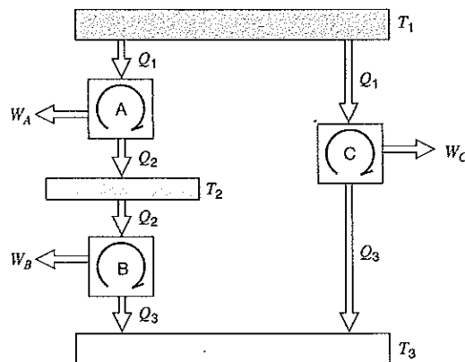
FIGURE 7.21 Arrangement of heat engines to demonstrate the thermodynamic temperature scale.
