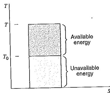
FIGURE 10.2 T - S diagram for constant- temperature energy source.
