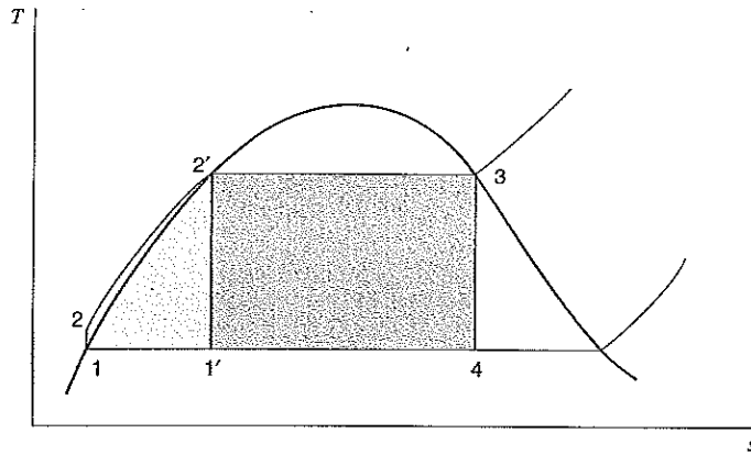
FIGURE 11.8 Temperature-entropy diagram showing the relationships between Carnot-cycle efficiency and Rankine-cycle efficiency.
