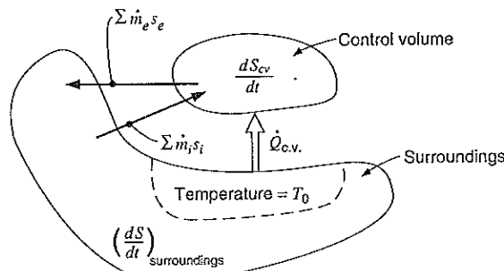
FIGURE 9.9 Entropy change for a control volume plus surroundings.
