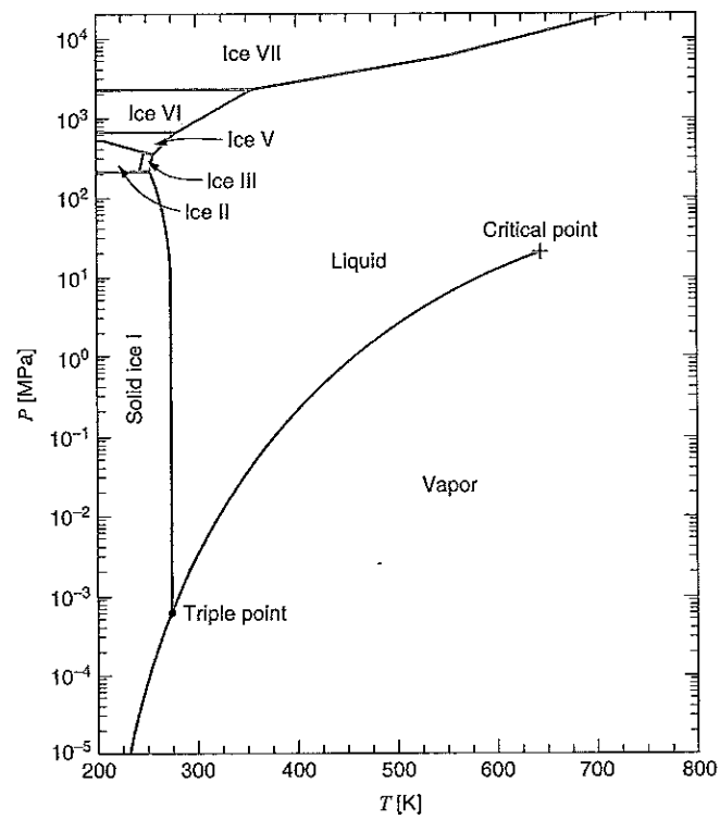
FIGURE 3.7 Water phase diagram.
