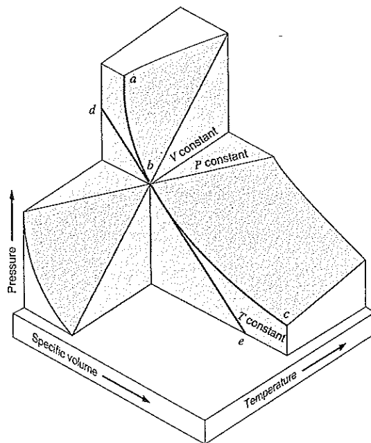
FIGURE 13.2 Schematic representation of partial derivatives.
