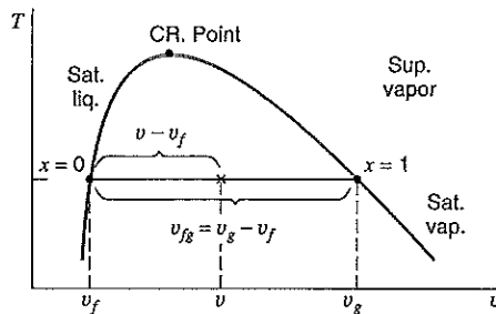
FIGURE 3.4 T - v diagram for the two-phase liquid-vapor region to show the quality specific volume relation.
