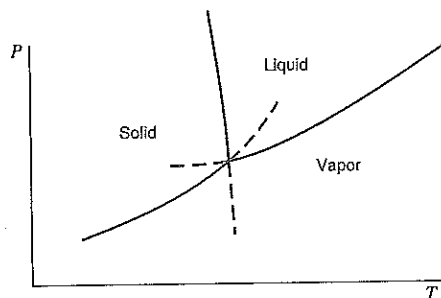
FIGURE 15.5 Metastable states for solid-liquid-vapor equilibrium.
