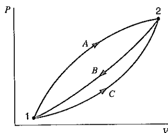
FIGURE 8.4 Two reversible cycles demonstrating the fact that entropy is a property of a substance.
