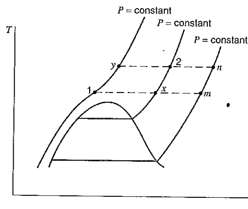
FIGURE 13.4 Sketch showing various paths by which a given change of state can take place.
