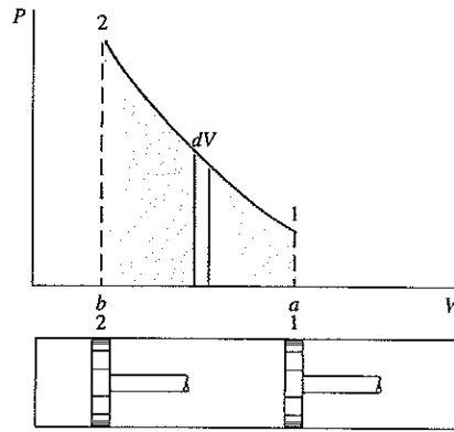
FIGURE 4.5 Use of pressure–volume diagram to show work done at the moving boundary of a system in a quasi-equilibrium process.
