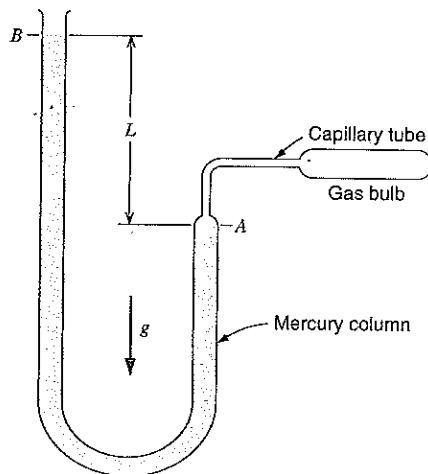
FIGURE 7.22 Schematic diagram of a constant-volume gas thermometer.
