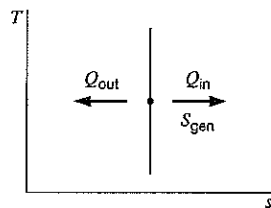
FIGURE 8.13 Change of entropy due to heat transfer and entropy generation.
