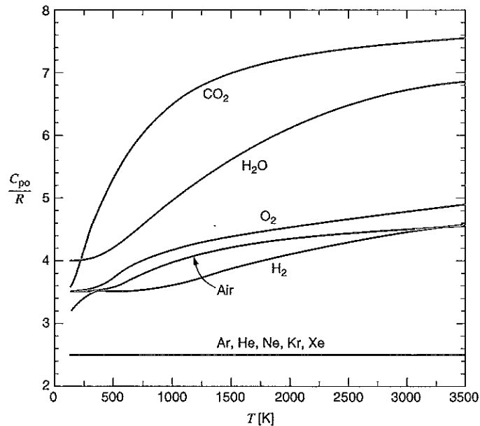
FIGURE 5.11 Heat capacity for some gases as function of temperature.
