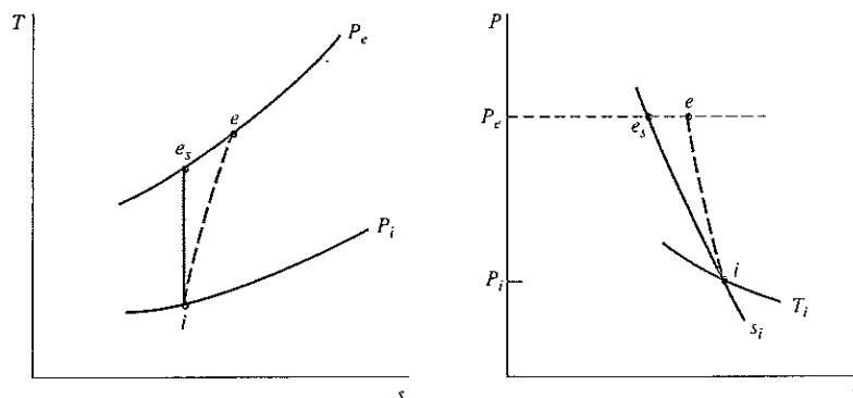
FIGURE 9.11 The compression process in an ideal and actual adiabatic compressor.
