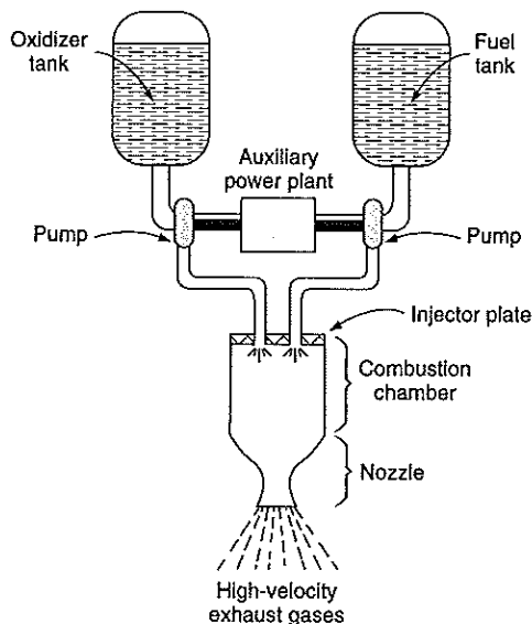
FIGURE 1.12 Simplified schematic diagram of a liquid- propellant rocket engine.
