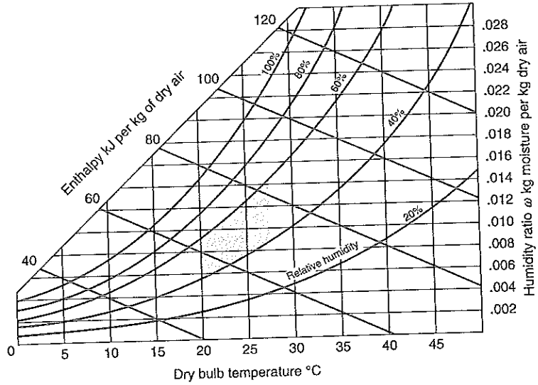
FIGURE 12.8 Psychrometric chart.
