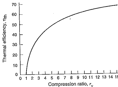
FIGURE 11.29 Thermal efficiency of the Otto cycle as a function of compression ratio.
