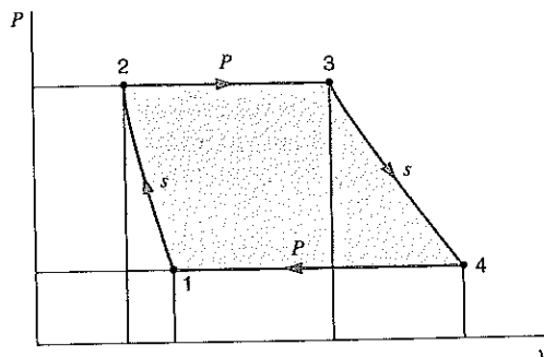
FIGURE 11.2 Four-process power cycle.
