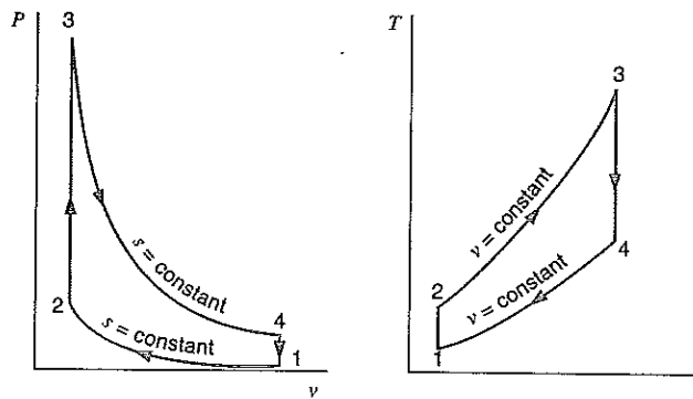
FIGURE 11.28 The air-standard Otto cycle.
