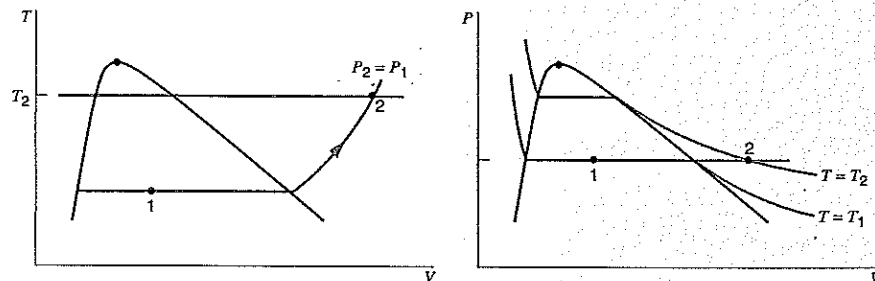
FIGURE 5.8 The constant-pressure quasi-equilibrium process.
