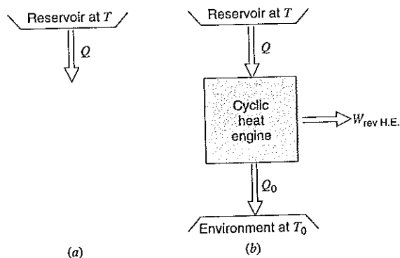
FIGURE 10.1 Constant-temperature energy source.
