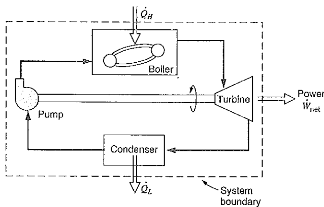
FIGURE 7.4 A heat engine involving steady-state processes.
