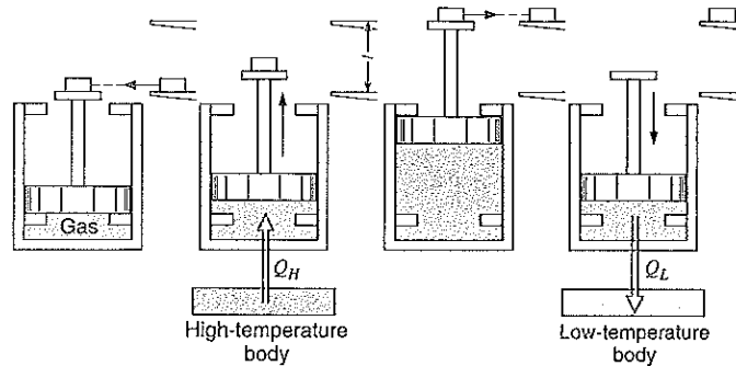
FIGURE 7.3 A simple heat engine.
