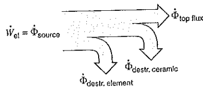
FIGURE 10.18 The fluxes and destruction terms of exergy.
