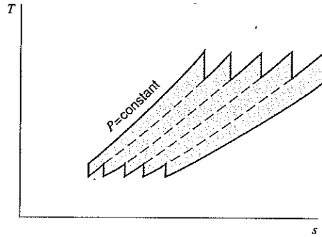
FIGURE 11.24 Temperature-entropy diagram that shows how the gas-turbine cycle with many stages approaches the Ericsson cycle.
