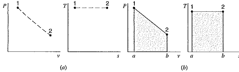
FIGURE 8.14 Reversible and irreversible processes on pressure–volume and temperature–entropy diagrams.
