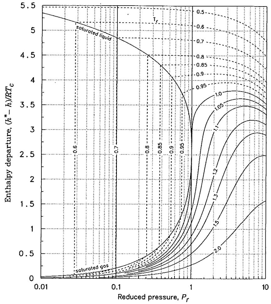
FIGURE D.2 Lee-Kesler Simple Fluid Enthalpy Departure.
