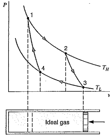
FIGURE 7.24 The ideal-gas Carnot cycle.
