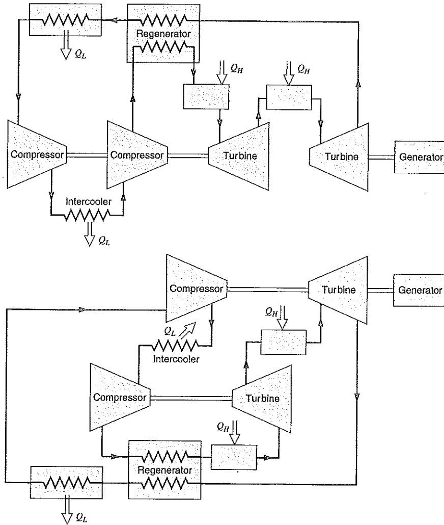
FIGURE 11.25 Some arrangements of components that may be utilized in stationary gas-turbine power plants.
