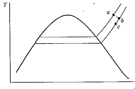
FIGURE 11.14 Temperature–entropy diagram showing effect of losses between boiler and turbine.
