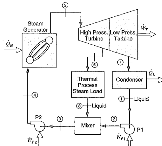
FIGURE 11.17 Example of a cogeneration system.
