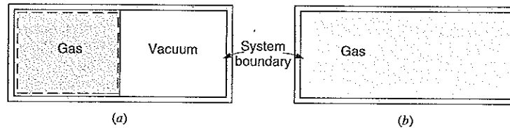
FIGURE 4.17 Example of process involving a change of volume for which the work is zero.
