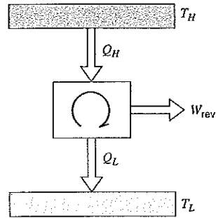
FIGURE 8.1 Reversible heat engine cycle for demonstration of the inequality of Clausius.
