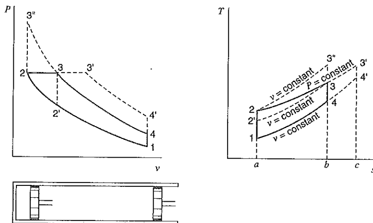
FIGURE 11.30 The air-standard diesel cycle.
