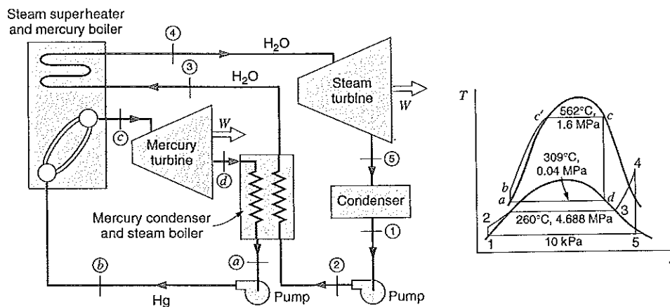
FIGURE 11.39 Mercury-water binary power system.
