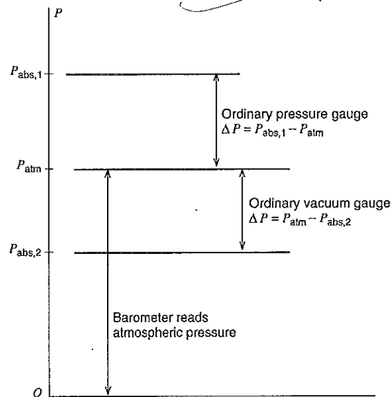
FIGURE 2.11 Illustration of terms used in pressure measurement.
