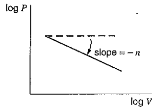
FIGURE 8.17 Example of a polytropic process.
