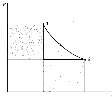
FIGURE 11.1 Comparison of shaft work and boundary-movement work.
