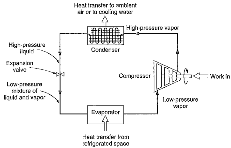
FIGURE 1.6 Schematic diagram of a simple refrigeration cycle.
