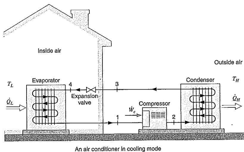
FIGURE 7.26 An air conditioner in cooling mode where T_L is the room.
