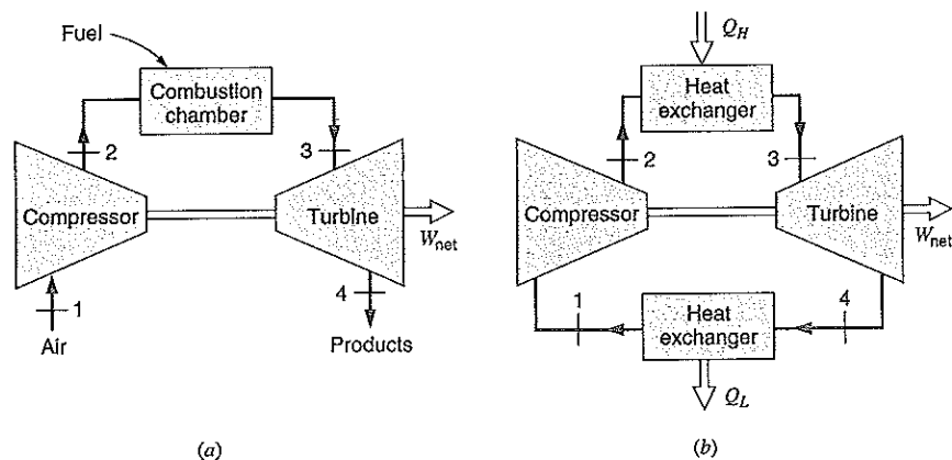
FIGURE 11.18 A gas turbine operating on the Brayton cycle. (a) Open cycle. (b) Closed cycle.
