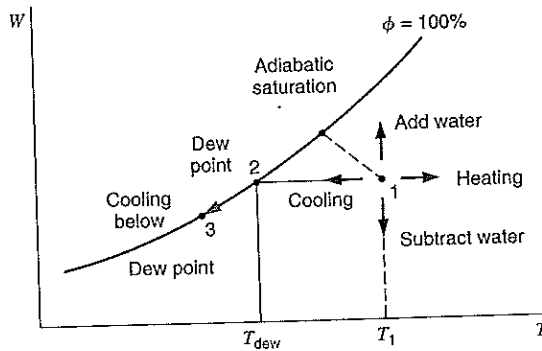
FIGURE 12.9 Processes on a psychrometric chart.
