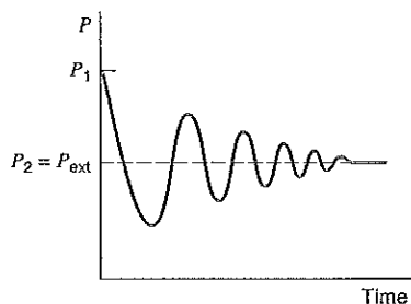
FIGURE 4.15 Cylinder pressure as a function of time.
