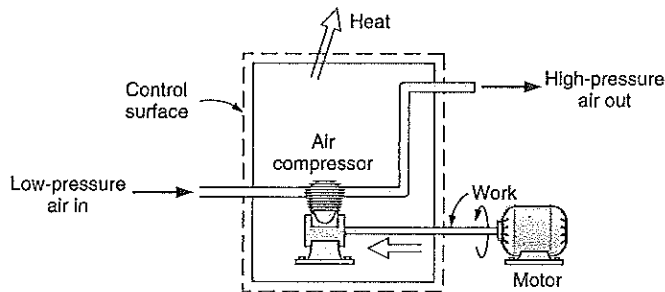
FIGURE 2.2 Example of a control volume.
