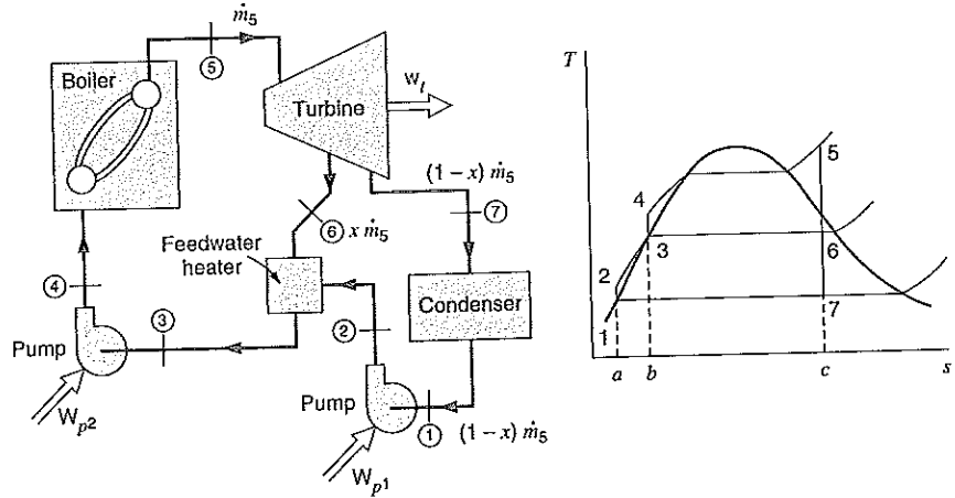
FIGURE 11.10 Regenerative cycle with open feedwater heater.
