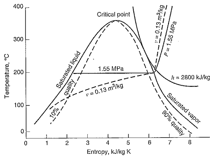
FIGURE 8.5 Temperature-entropy diagram for steam.
