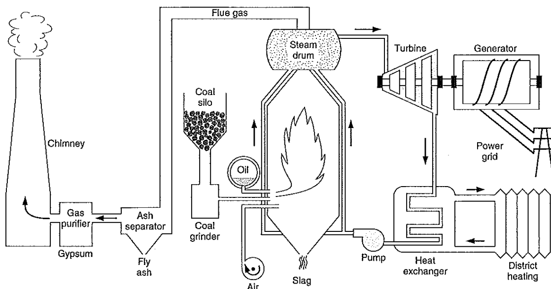
FIGURE 1.1 Schematic diagram of a steam power plant.
