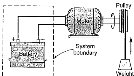
FIGURE 4.2 Example of work crossing the boundary of a system because of a flow of an electric current across the system boundary.
