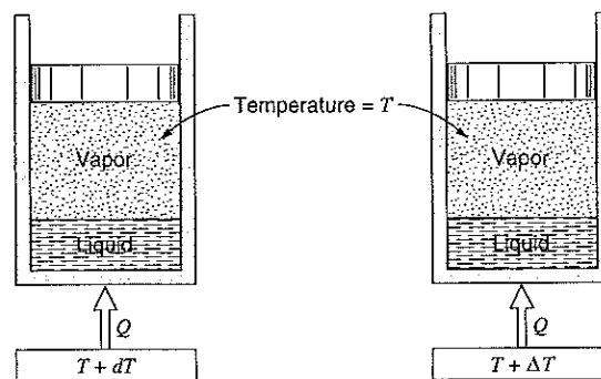
FIGURE 7.17 Illustration of the difference between an internally and externally reversible process.
