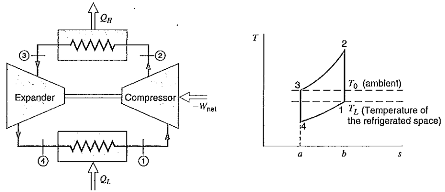
FIGURE 11.36 The air-standard refrigeration cycle.
