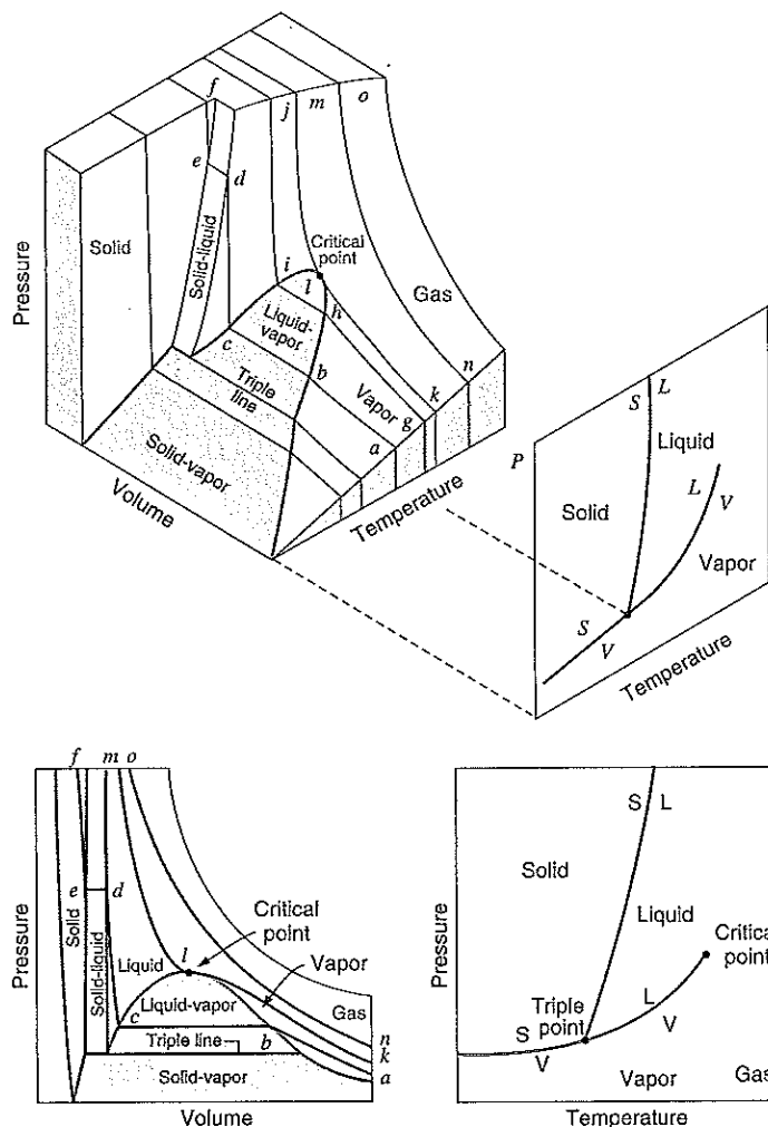
FIGURE 3.19 Pressure–volume–temperature surface for a substance that contracts on freezing.
