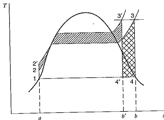
FIGURE 11.6 Effect of boiler pressure on Rankine-cycle efficiency.
