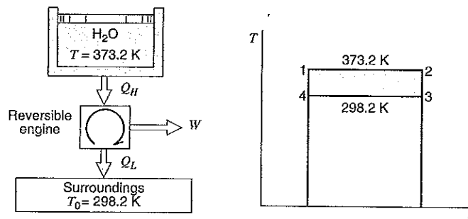
FIGURE 8.16 Reversible heat transfer with the surroundings.
