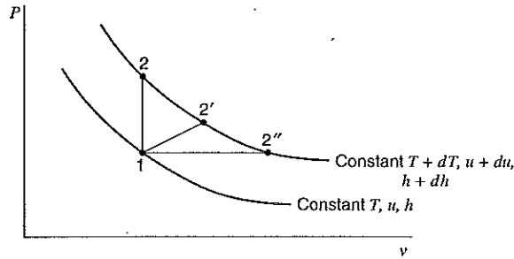
FIGURE 5.10 Pressure–volume diagram for an ideal gas.
