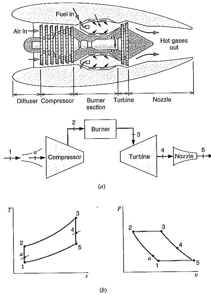
FIGURE 11.26 The ideal gas-turbine cycle for a jet engine.
