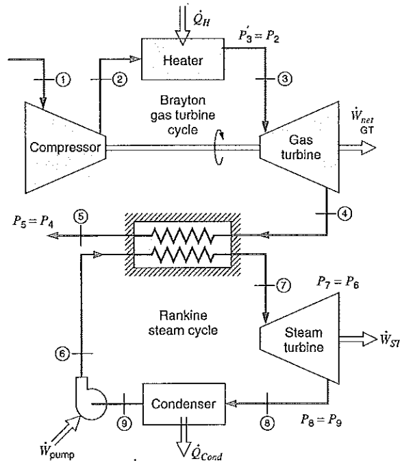
FIGURE 11.40 Combined Brayton/Rankine cycle power system.
