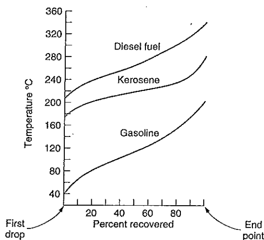
FIGURE 14.2 Typical distillation curves of some hydrocarbon fuels.
