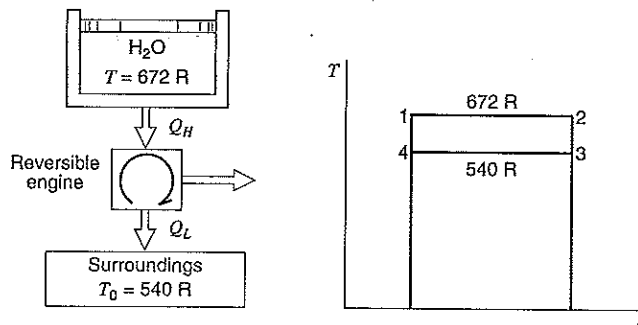
FIGURE 8.16E Reversible heat transfer with the surroundings.
