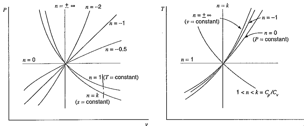
FIGURE 8.18 Polytropic process on P - v and T - s diagrams.
