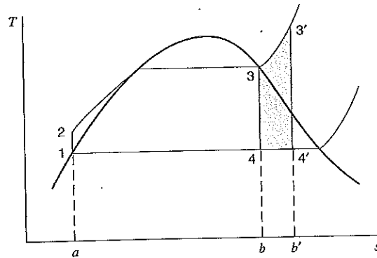
FIGURE 11.5 Effect of superheating on Rankine-cycle efficiency.
