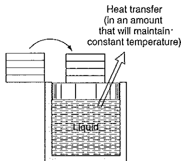
FIGURE 3.9 Illustration of compressed-liquid state.
