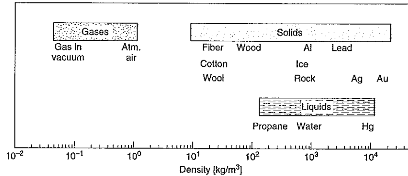
FIGURE 2.7 Density of common substances.
