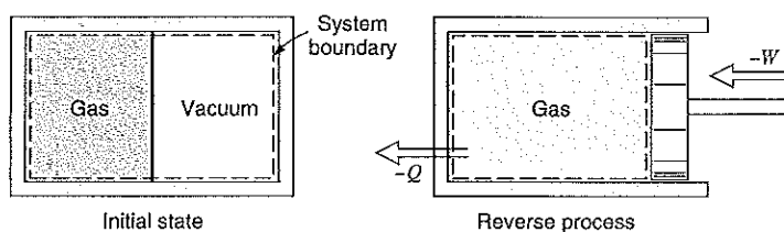
FIGURE 7.15 Demonstration of the fact that unrestrained expansion makes processes irreversible.
