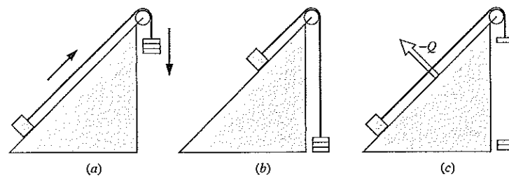
FIGURE 7.14 Demonstration of the fact that friction makes processes irreversible.
