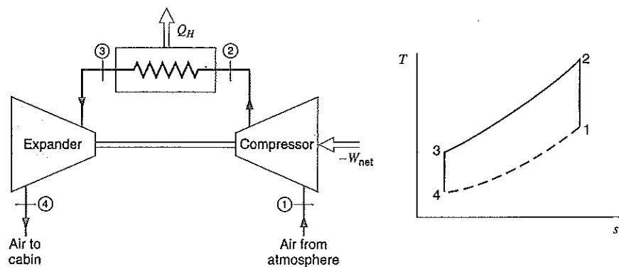
FIGURE 11.37 An air refrigeration cycle that might be utilized for aircraft cooling.
