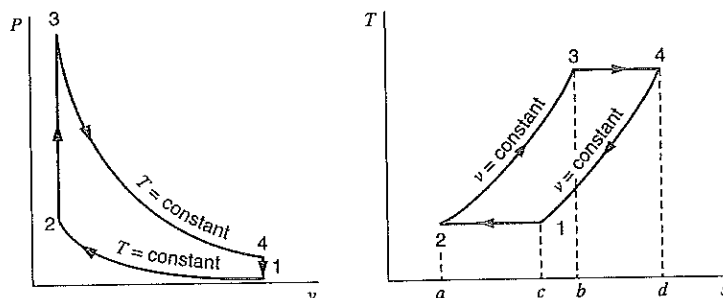
FIGURE 11.31 The air-standard Stirling cycle.
