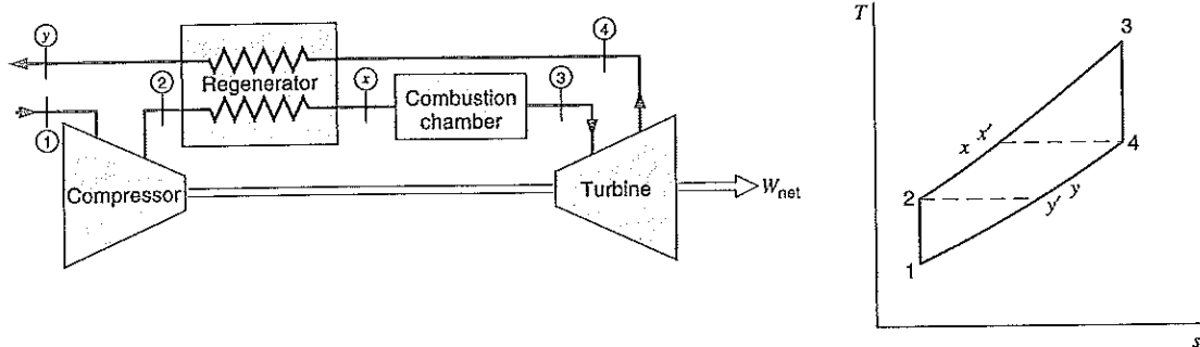
FIGURE 11.22 Temperature-entropy diagram to illustrate the definition of regenerator efficiency.
