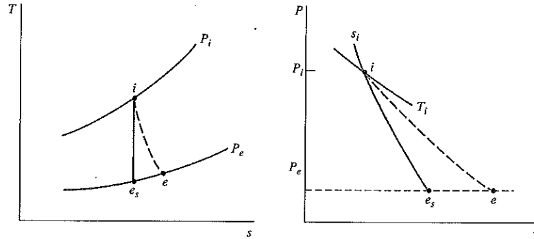
FIGURE 9.12 The ideal and actual process in an adiabatic nozzle.
