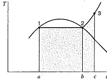
FIGURE 8.9 A temperature–entropy diagram to show areas that represent heat transfer for an internally reversible process.
