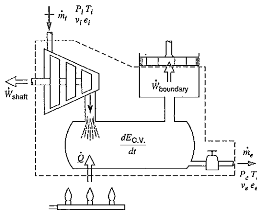
FIGURE 6.4 Schematic diagram to illustrate terms in the energy equation for a general control volume.
