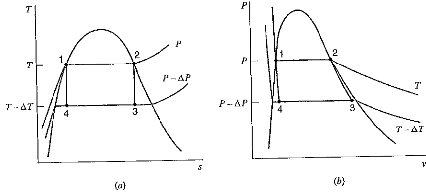
FIGURE 13.1 A Carnot cycle operating across a small temperature difference.
