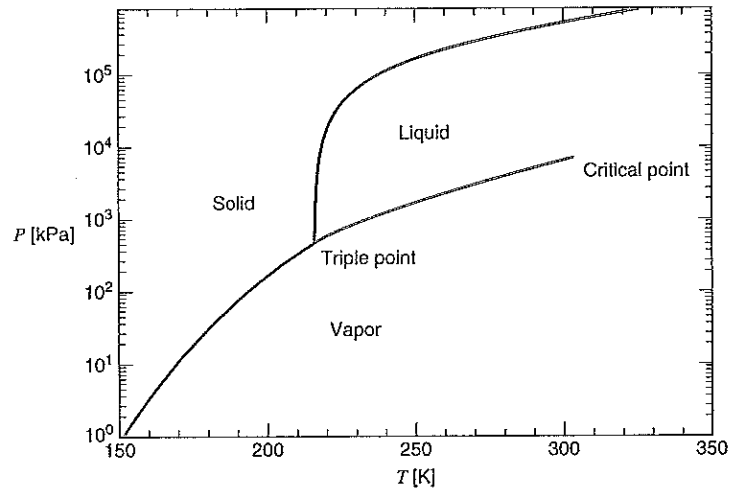
FIGURE 3.6 Carbon dioxide phase diagram.
