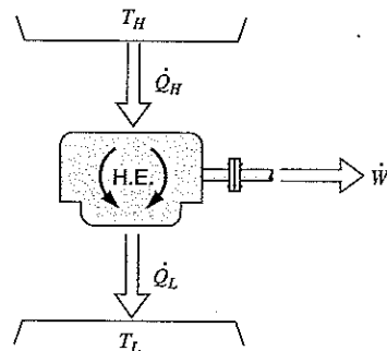
FIGURE 7.25 A heat engine operating between two constant temperature energy reservoirs for Example 7.1.
