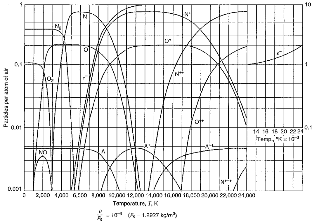
FIGURE 15.11 Equilibrium composition of air [W. E. Moeckel and K. C. Weston, NACA TN 4265 (1958)].
