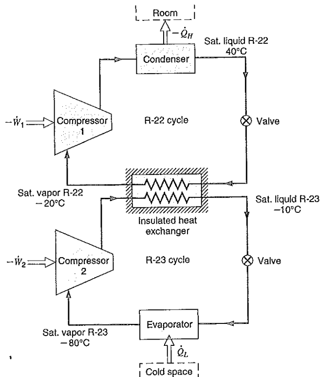
FIGURE 11.41 Combined-cycle cascade refrigeration system.
