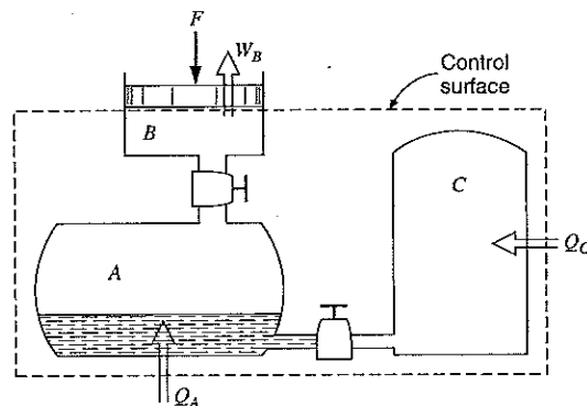
FIGURE 5.3 A control mass with several different subsystems.
