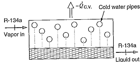
FIGURE 6.5 A refrigeration system condenser.
