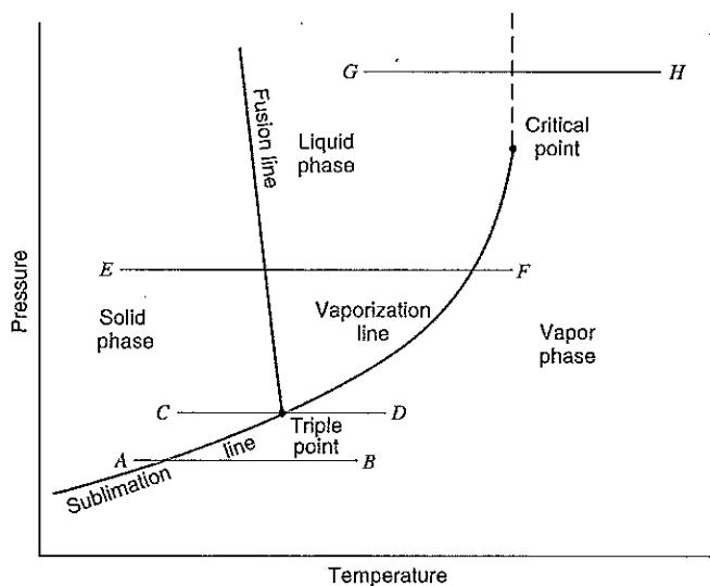
FIGURE 3.5 Pressure-temperature diagram for a substance such as water.
