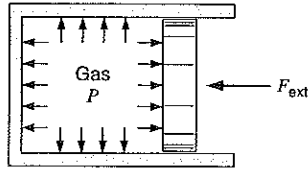
FIGURE 2.9 The balance of forces on a movable boundary relates to inside gas pressure.
