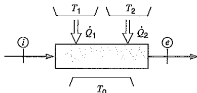
FIGURE 10.6 The feedwater heater for Example 10.1.
